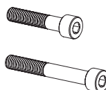
2 x M8 40mm BOLTS 2 x M8 60mm BOLTS
